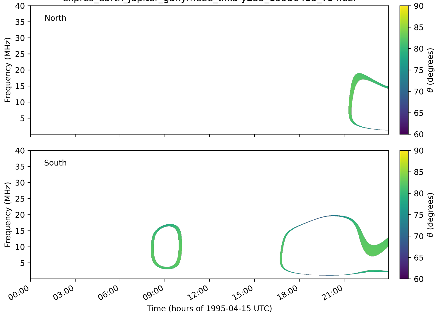
expres_earth_jupiter_ganymede_txka-y235_19950415_v14.cdf
