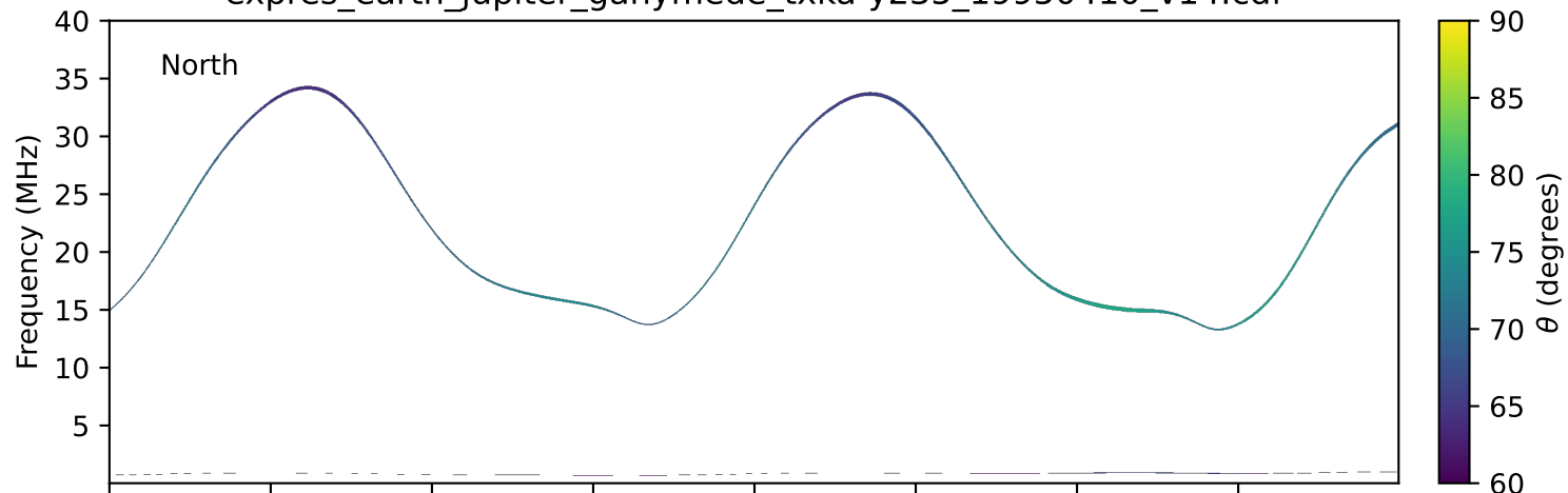
expres_earth_jupiter_ganymede_txka-y235_19950410_v14.cdf
