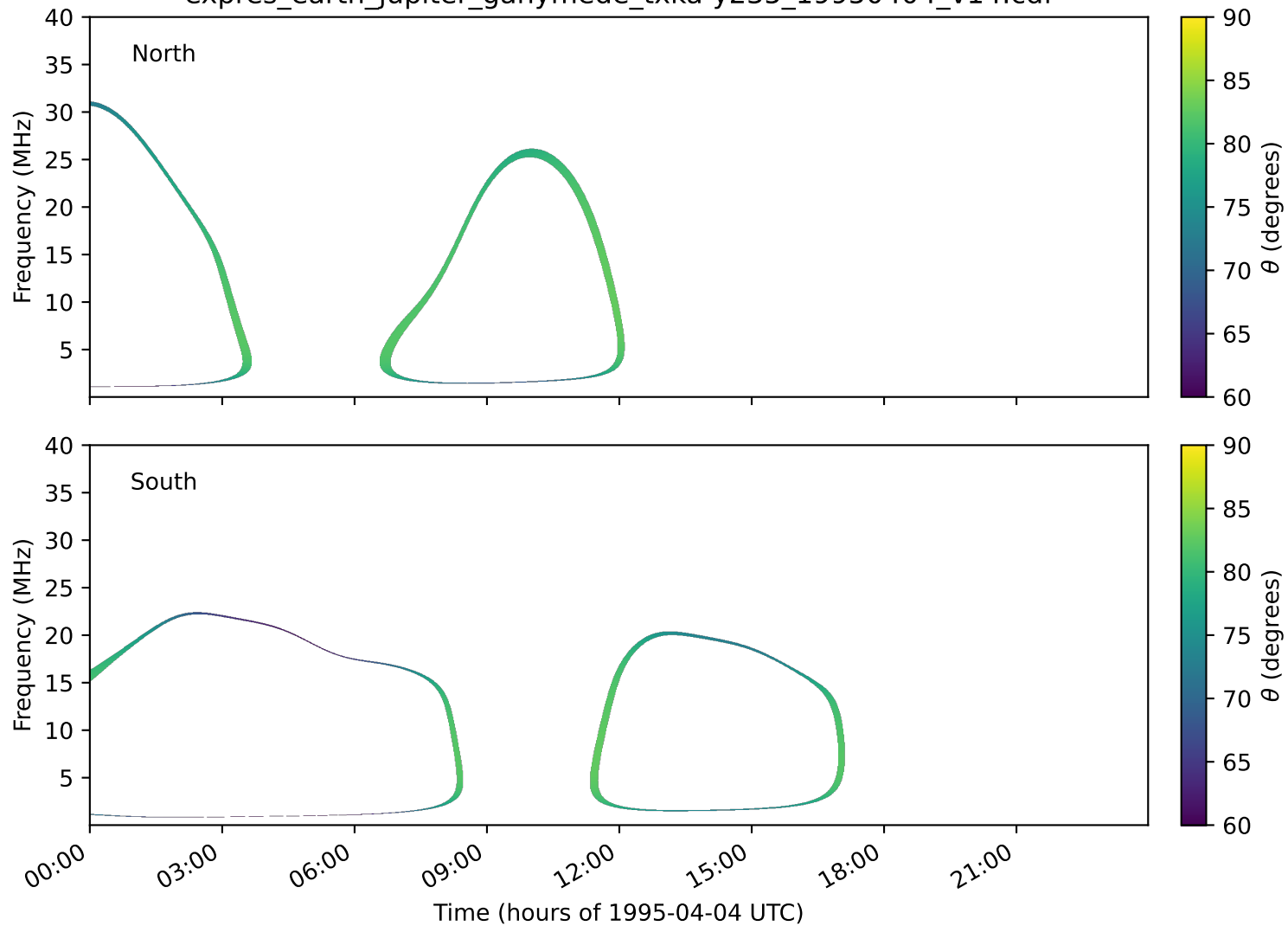
expres_earth_jupiter_ganymede_txka-y235_19950404_v14.cdf
