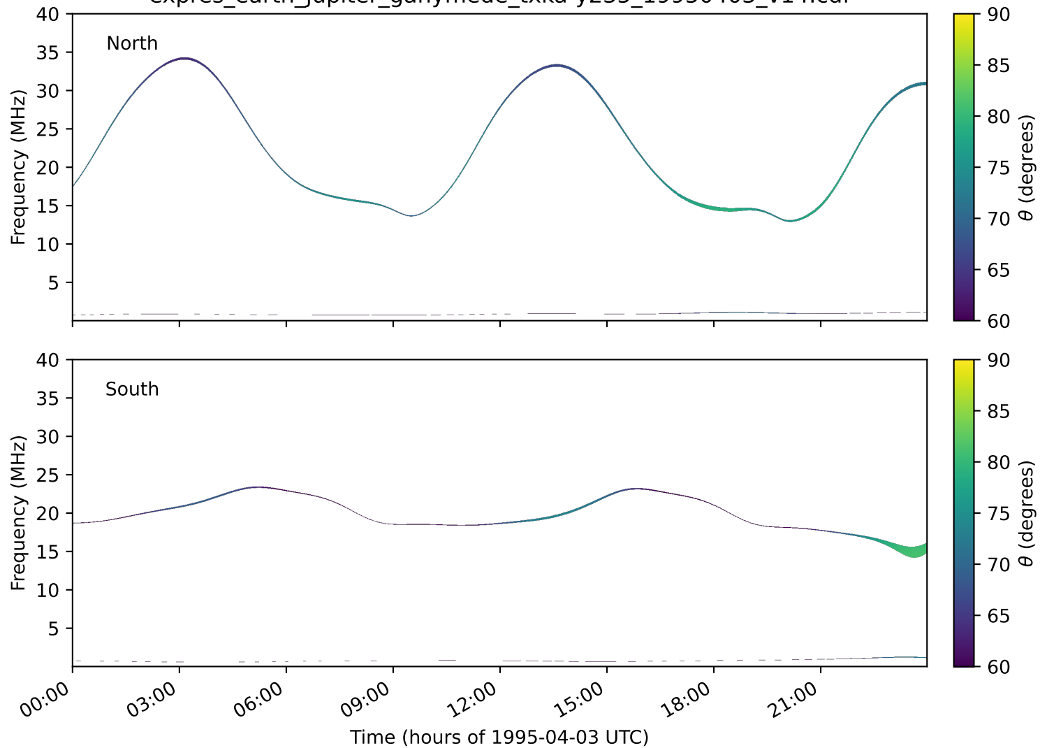
expres_earth_jupiter_ganymede_txka-y235_19950403_v14.cdf
