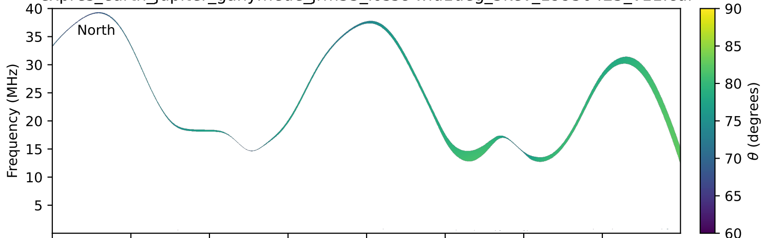
expres_earth_jupiter_ganymede_jrm33_lossc-wid1deg_3kev_19950425_v11.cdf
