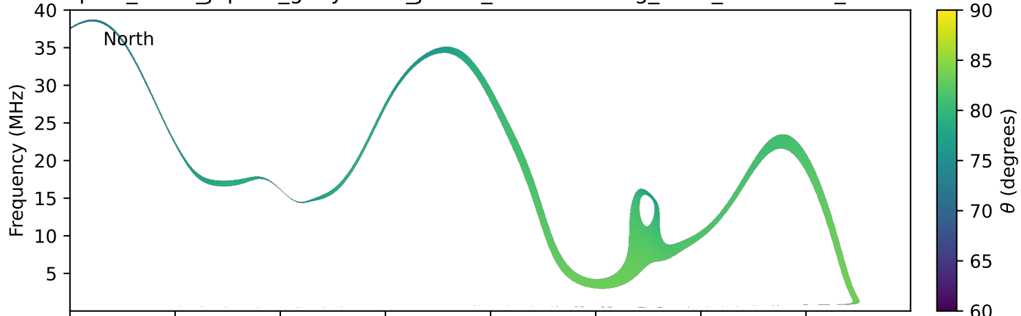
expres_earth_jupiter_ganymede_jrm33_lossc-wid1deg_3kev_19950411_v11.cdf
