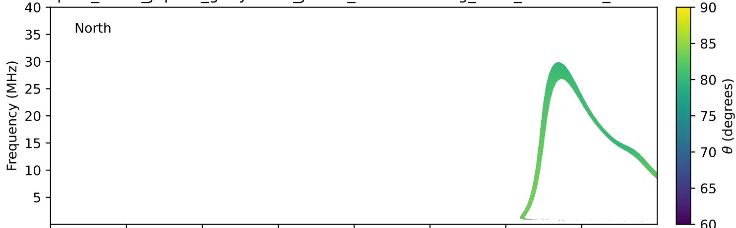
expres_earth_jupiter_ganymede_jrm33_lossc-wid1deg_3kev_19950401_v11.cdf
