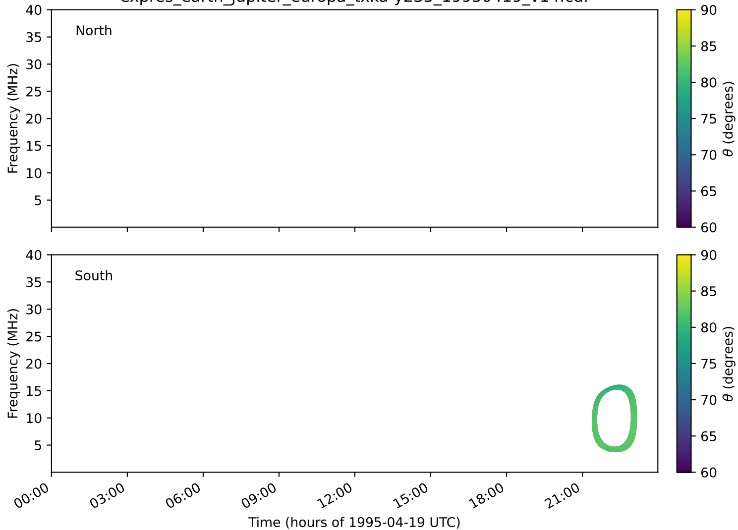
expres_earth_jupiter_europa_txka-y235_19950419_v14.cdf
