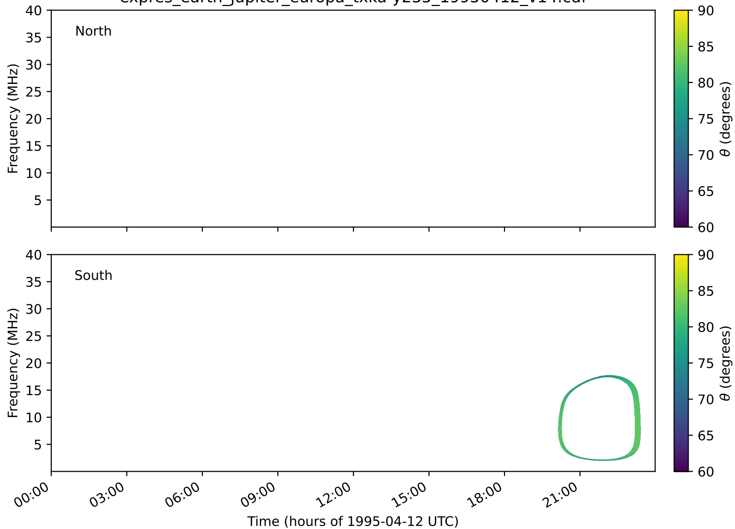
expres_earth_jupiter_europa_txka-y235_19950412_v14.cdf
