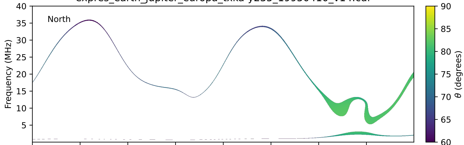
expres_earth_jupiter_europa_txka-y235_19950410_v14.cdf
