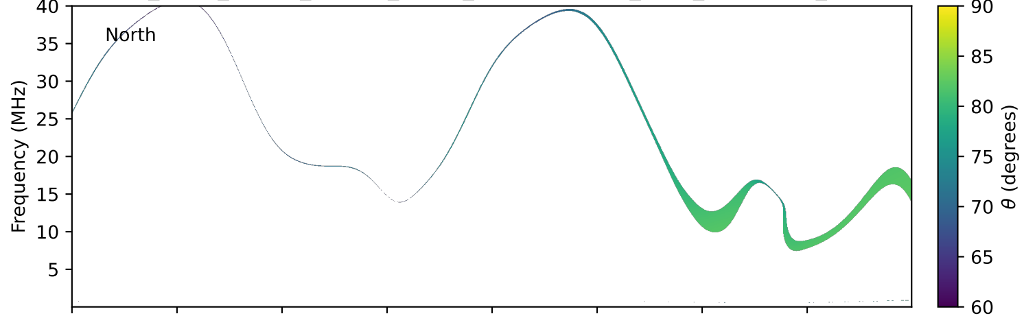
expres_earth_jupiter_europa_jrm33_lossc-wid1deg_3kev_19950403_v11.cdf
