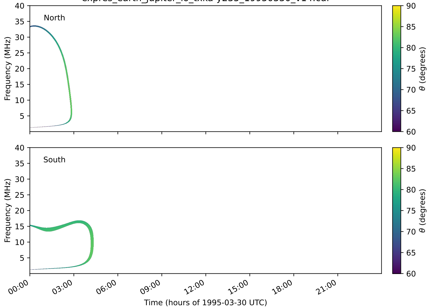
expres_earth_jupiter_io_txka-y235_19950330_v14.cdf
