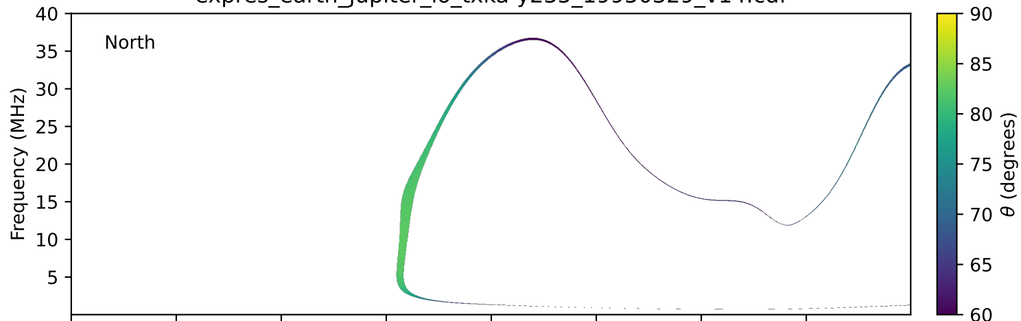
expres_earth_jupiter_io_txka-y235_19950329_v14.cdf
