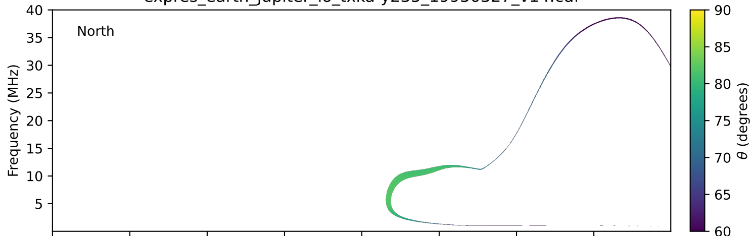
expres_earth_jupiter_io_txka-y235_19950327_v14.cdf
