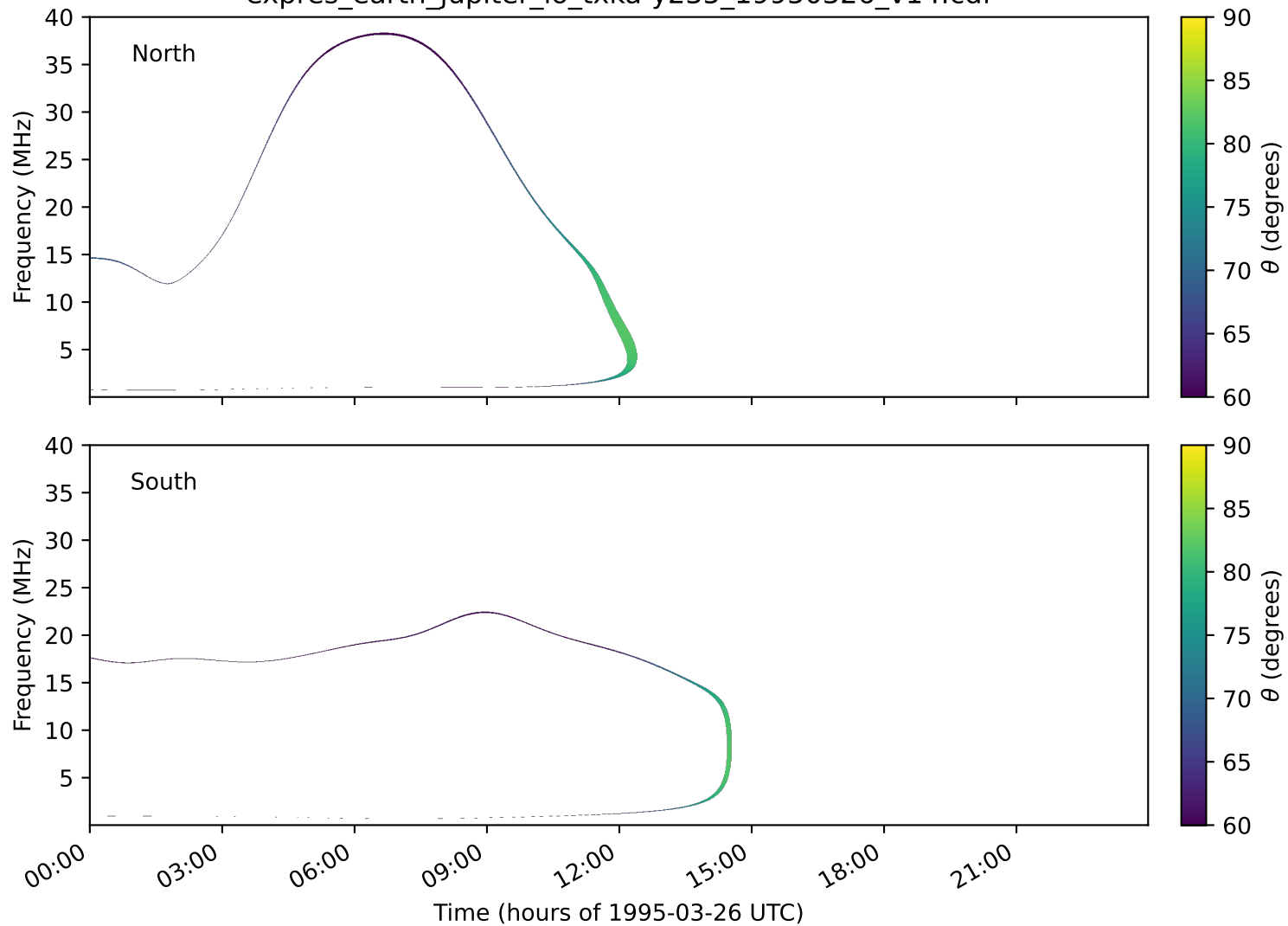
expres_earth_jupiter_io_txka-y235_19950326_v14.cdf
