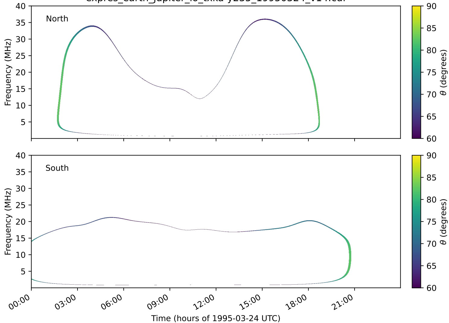
expres_earth_jupiter_io_txka-y235_19950324_v14.cdf
