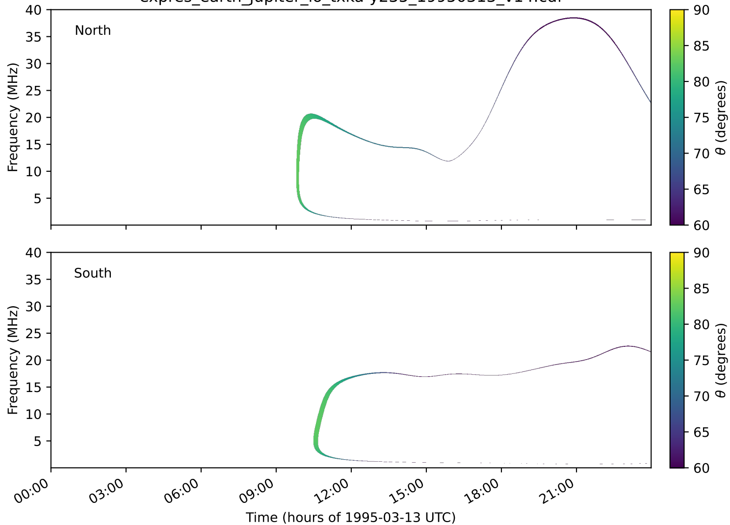
expres_earth_jupiter_io_txka-y235_19950313_v14.cdf
