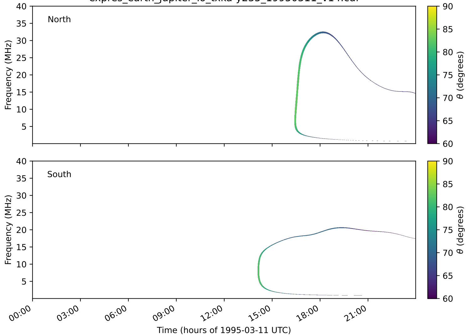
expres_earth_jupiter_io_txka-y235_19950311_v14.cdf
