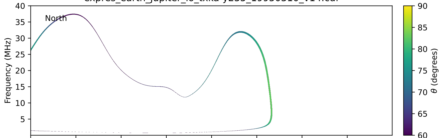
expres_earth_jupiter_io_txka-y235_19950310_v14.cdf
