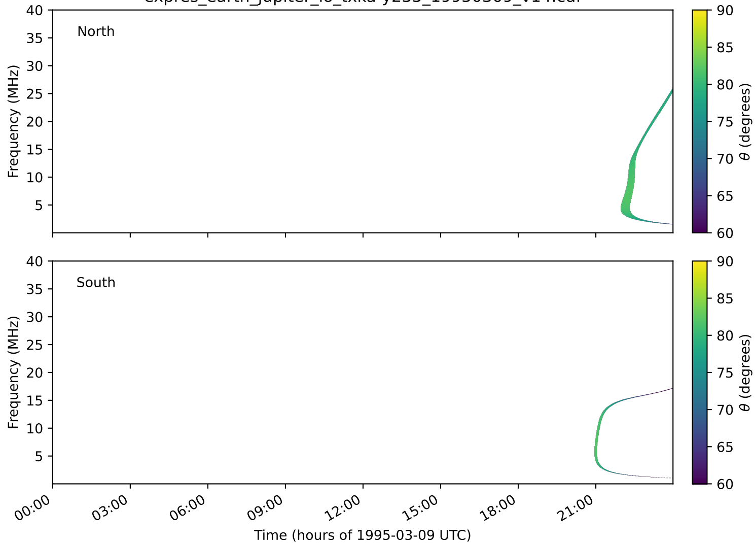
expres_earth_jupiter_io_txka-y235_19950309_v14.cdf
