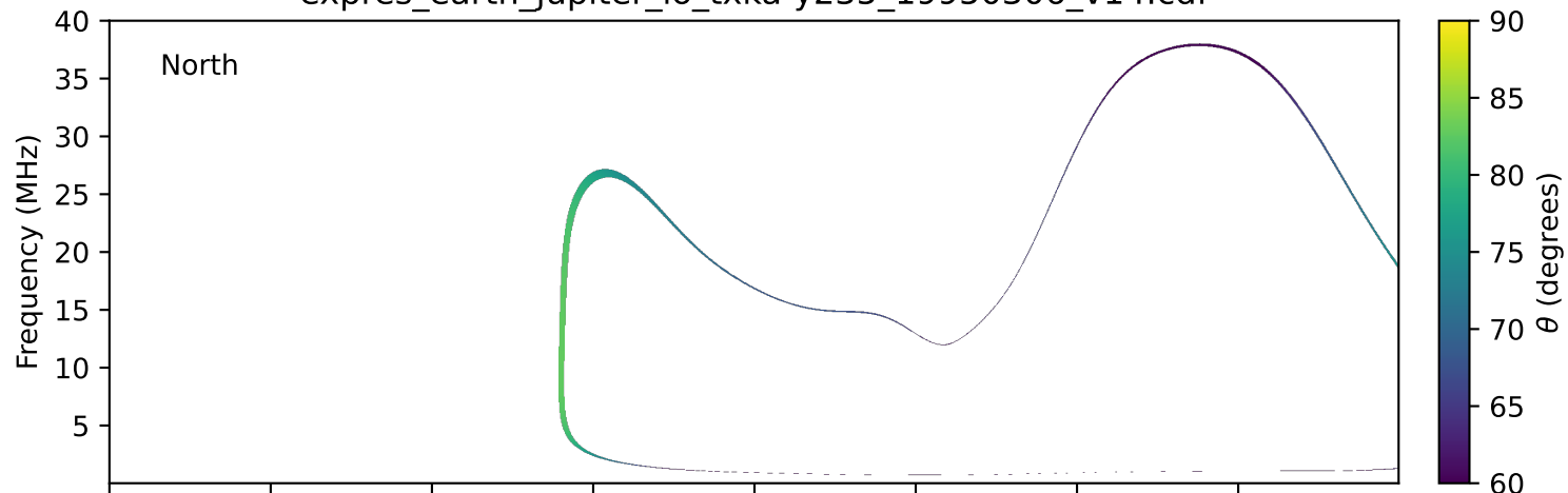
expres_earth_jupiter_io_txka-y235_19950306_v14.cdf
