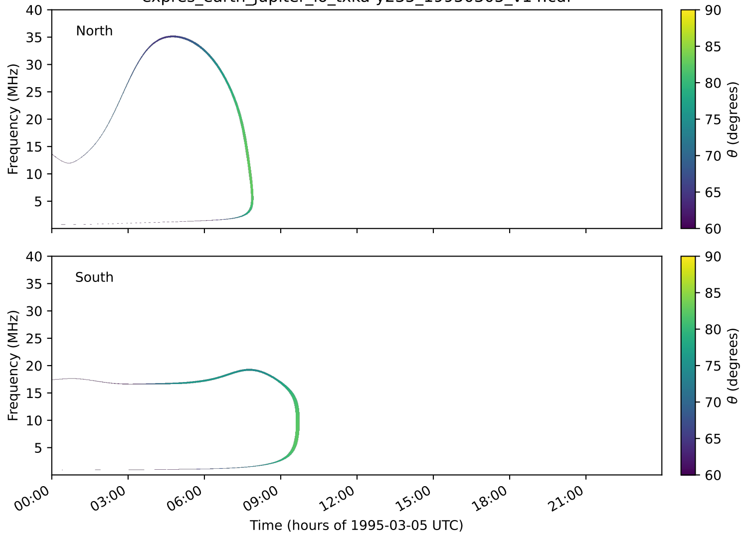
expres_earth_jupiter_io_txka-y235_19950305_v14.cdf
