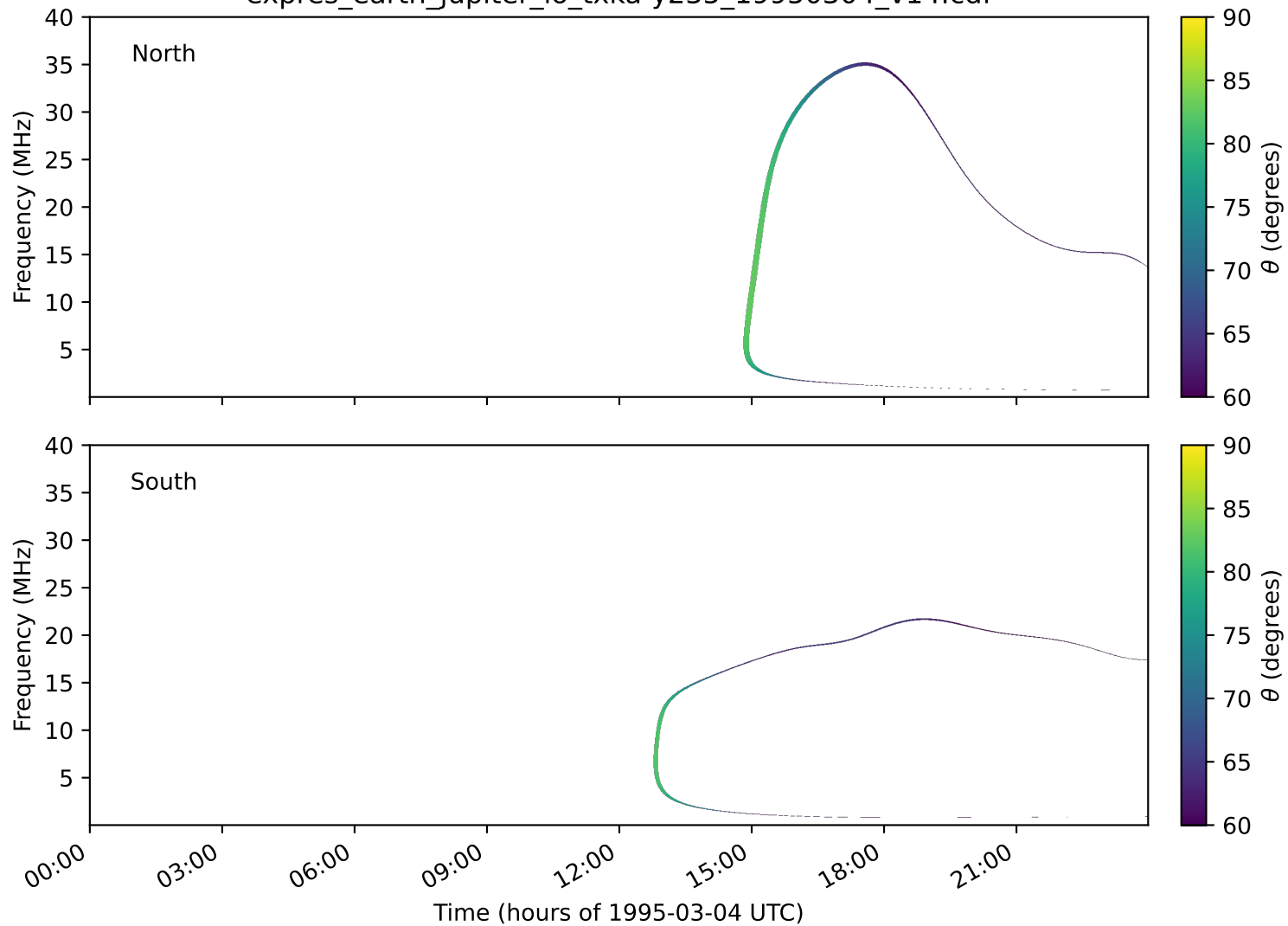
expres_earth_jupiter_io_txka-y235_19950304_v14.cdf
