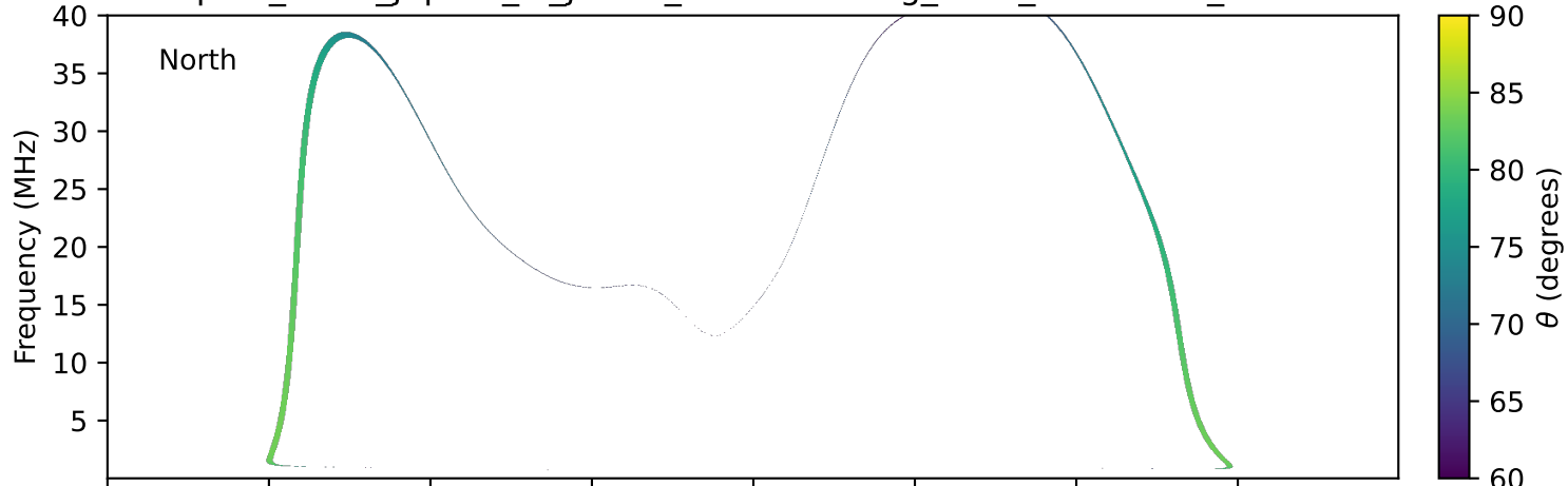
expres_earth_jupiter_io_jrm33_lossc-wid1deg_3kev_19950331_v11.cdf
