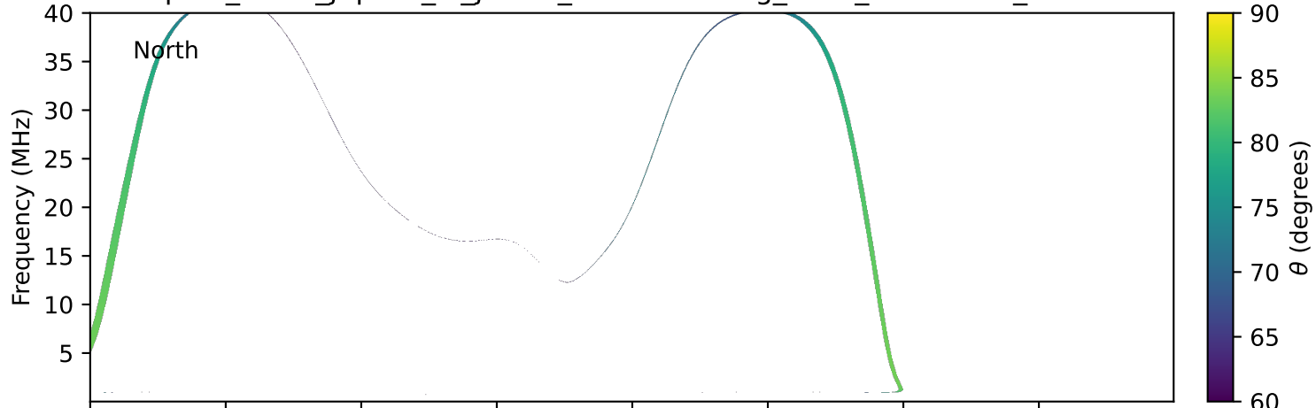
expres_earth_jupiter_io_jrm33_lossc-wid1deg_3kev_19950317_v11.cdf
