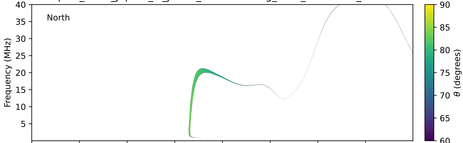
expres_earth_jupiter_io_jrm33_lossc-wid1deg_3kev_19950313_v11.cdf
