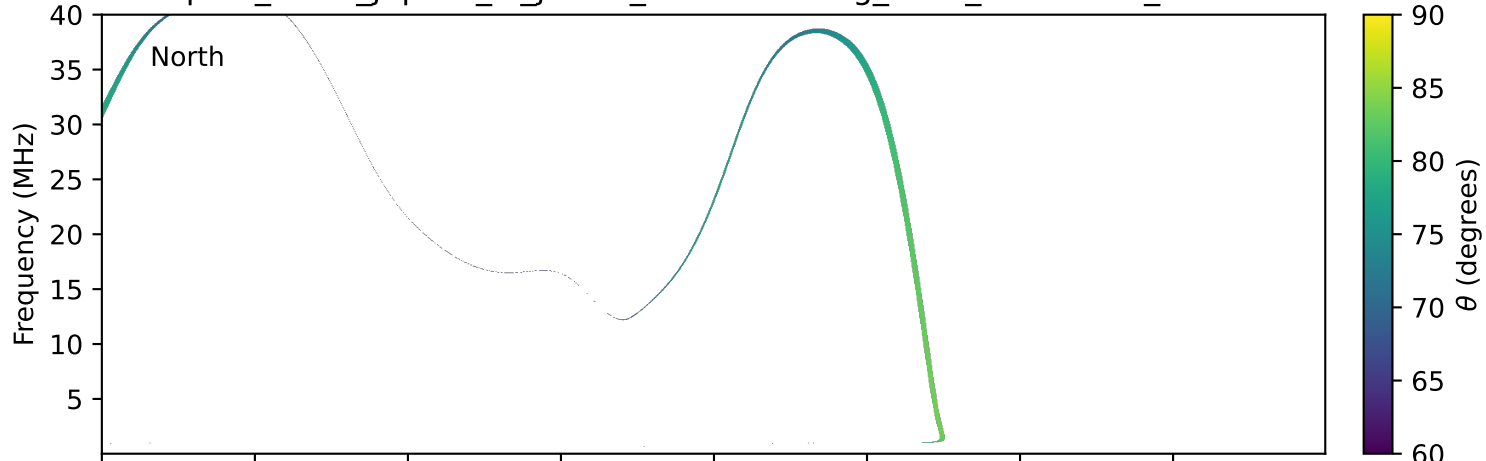
expres_earth_jupiter_io_jrm33_lossc-wid1deg_3kev_19950310_v11.cdf
