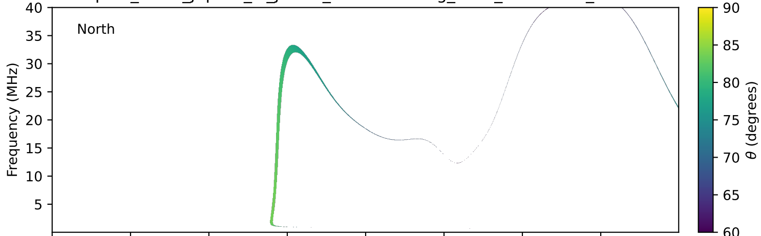
expres_earth_jupiter_io_jrm33_lossc-wid1deg_3kev_19950306_v11.cdf
