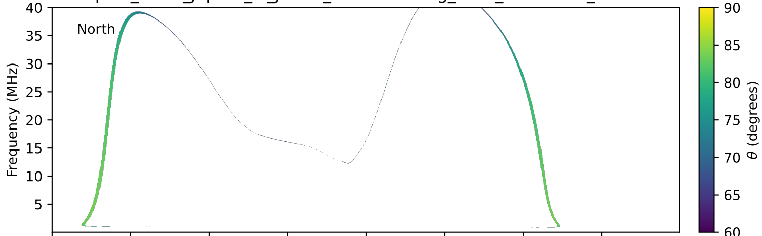
expres_earth_jupiter_io_jrm09_lossc-wid1deg_3kev_19950324_v11.cdf
