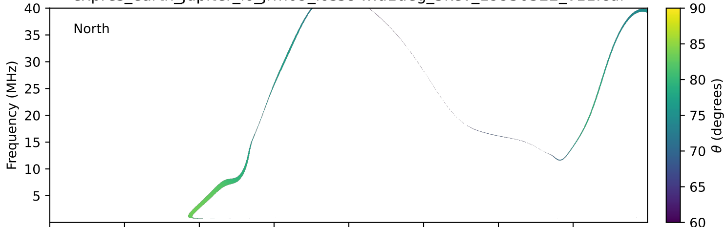
expres_earth_jupiter_io_jrm09_lossc-wid1deg_3kev_19950322_v11.cdf
