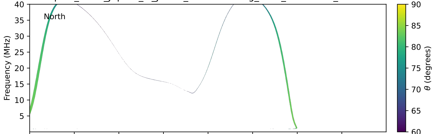
expres_earth_jupiter_io_jrm09_lossc-wid1deg_3kev_19950317_v11.cdf
