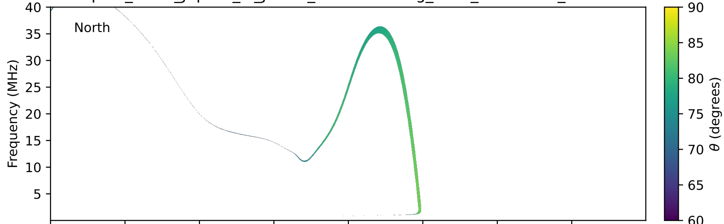
expres_earth_jupiter_io_jrm09_lossc-wid1deg_3kev_19950303_v11.cdf
