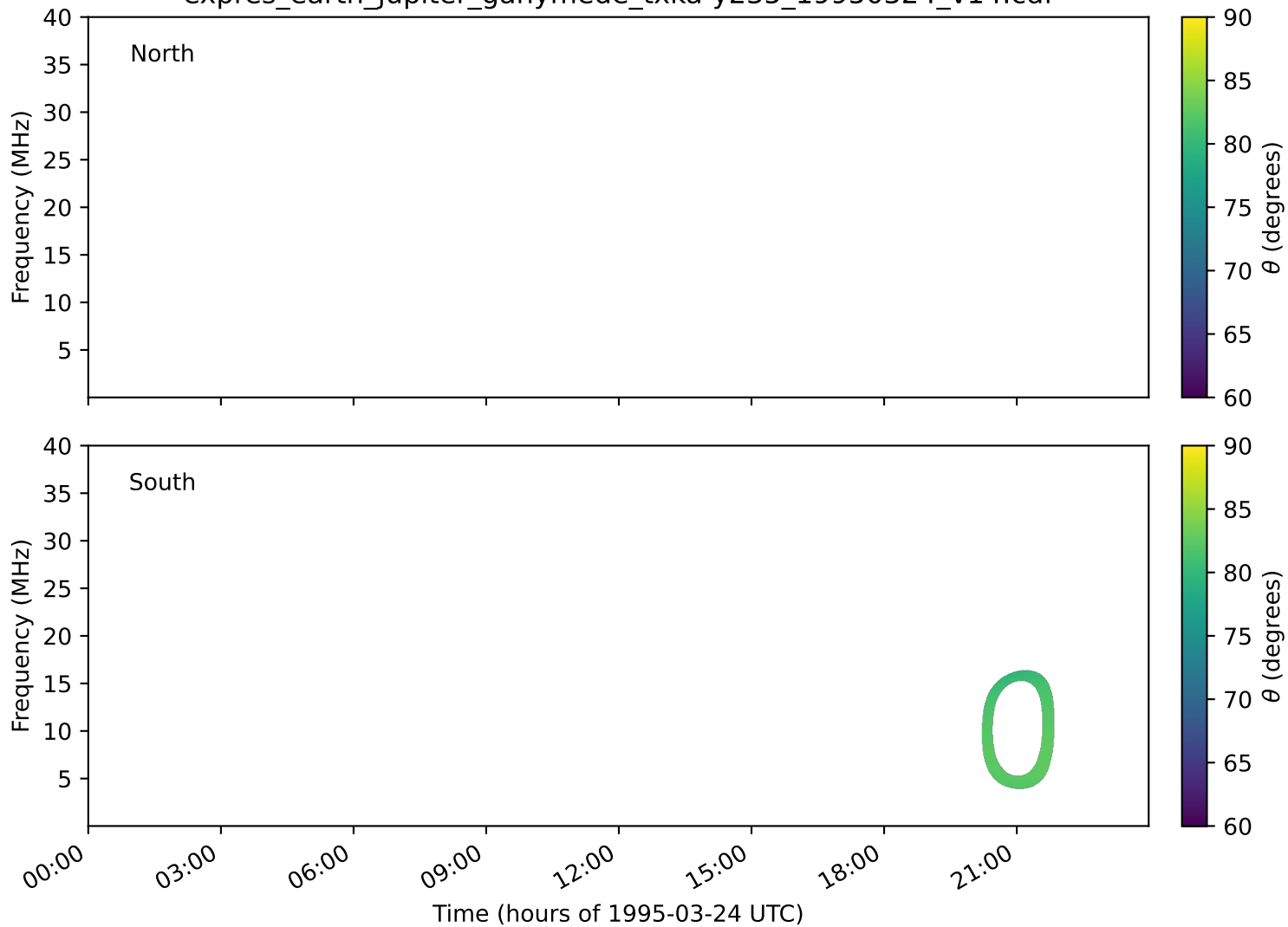
expres_earth_jupiter_ganymede_txka-y235_19950324_v14.cdf
