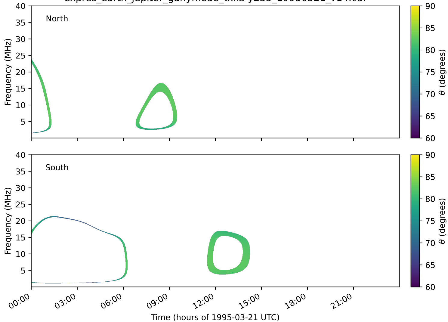
expres_earth_jupiter_ganymede_txka-y235_19950321_v14.cdf
