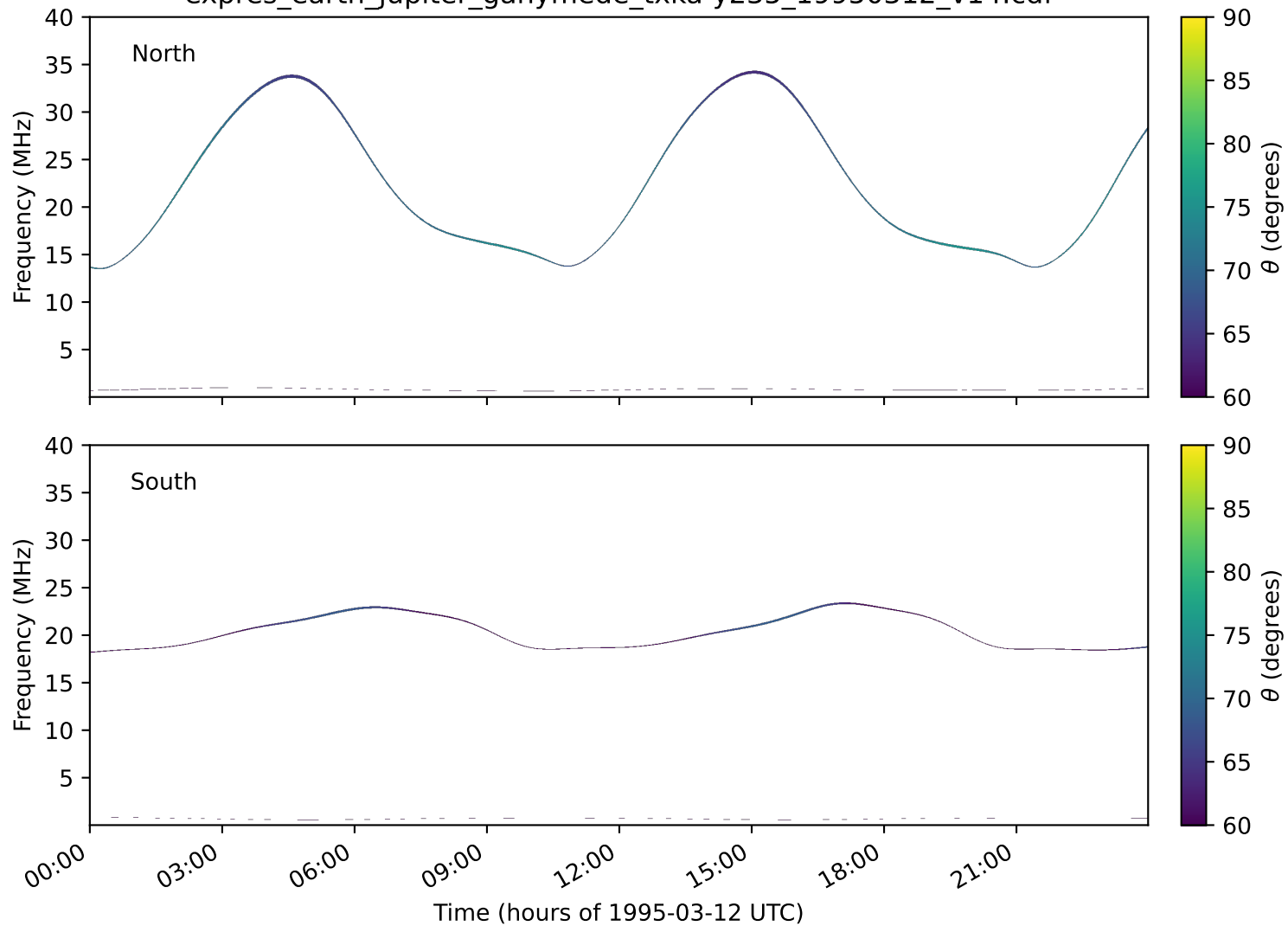
expres_earth_jupiter_ganymede_txka-y235_19950312_v14.cdf
