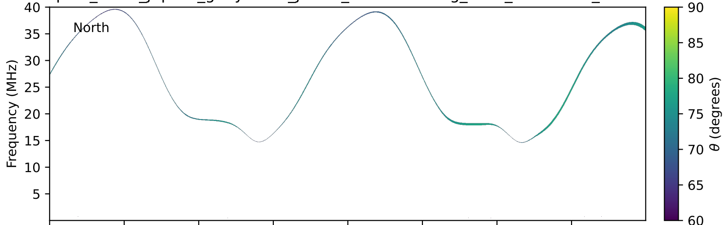
expres_earth_jupiter_ganymede_jrm33_lossc-wid1deg_3kev_19950327_v11.cdf
