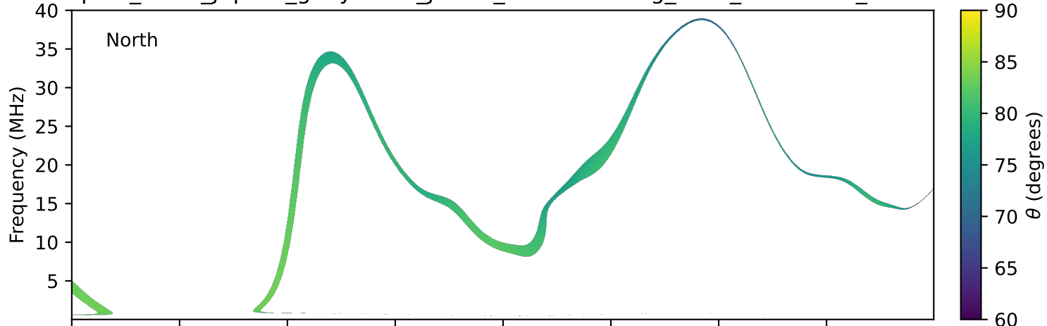
expres_earth_jupiter_ganymede_jrm33_lossc-wid1deg_3kev_19950304_v11.cdf
