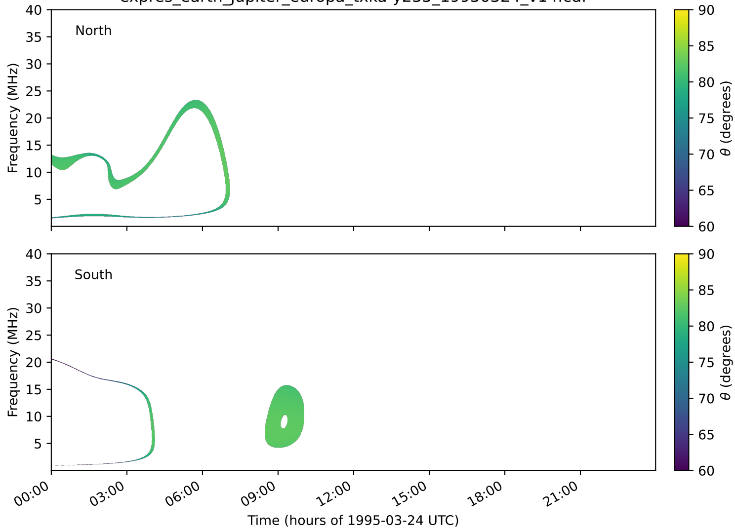
expres_earth_jupiter_europa_txka-y235_19950324_v14.cdf
