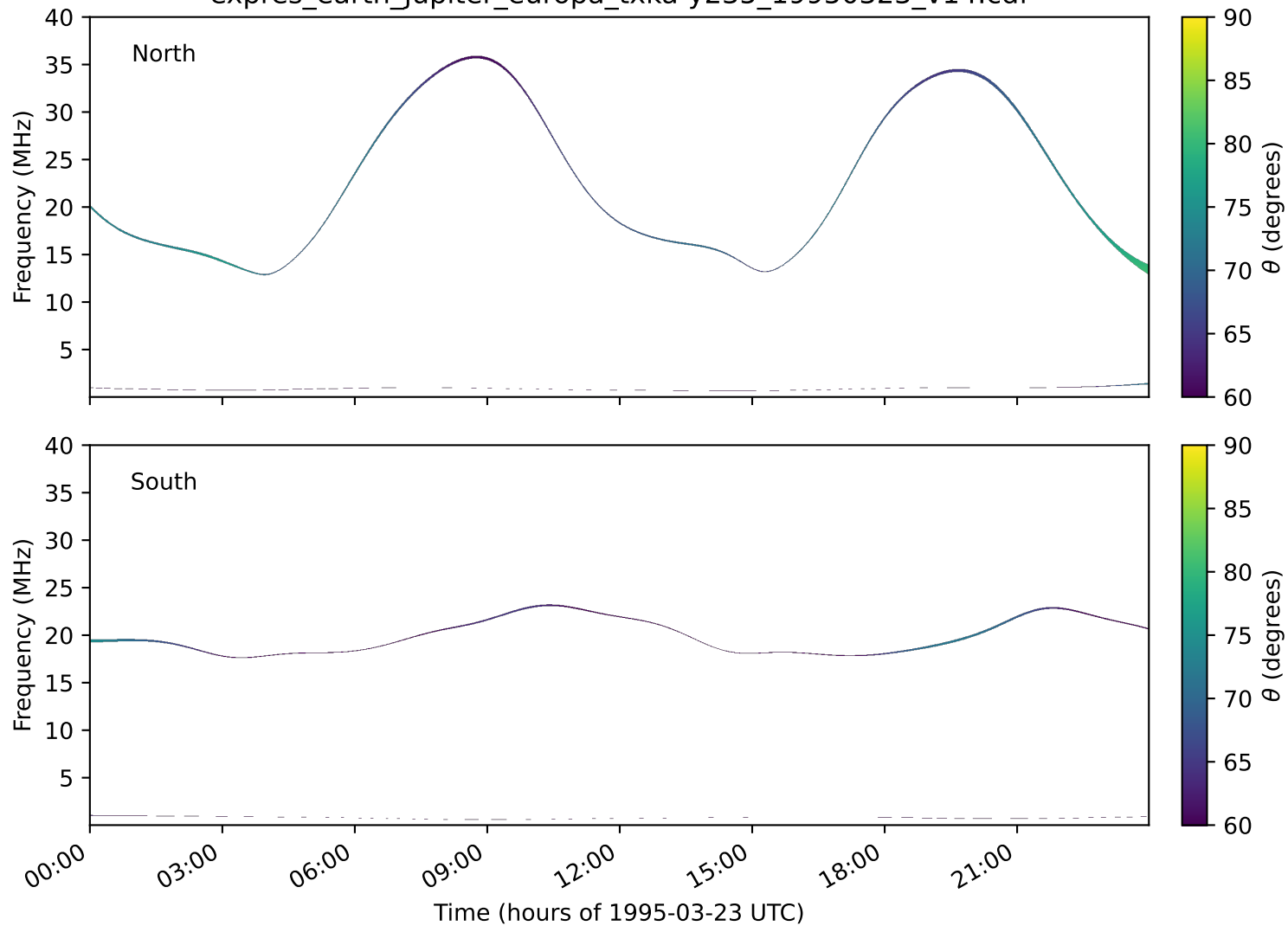
expres_earth_jupiter_europa_txka-y235_19950323_v14.cdf
