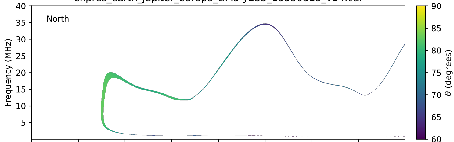
expres_earth_jupiter_europa_txka-y235_19950319_v14.cdf
