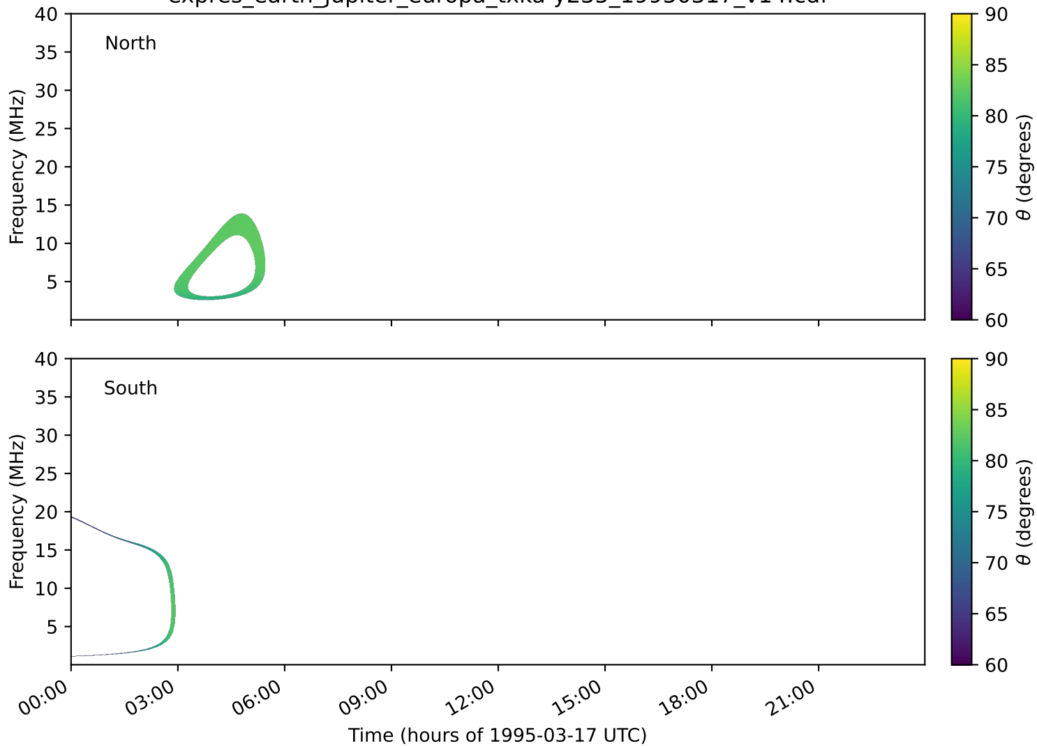
expres_earth_jupiter_europa_txka-y235_19950317_v14.cdf
