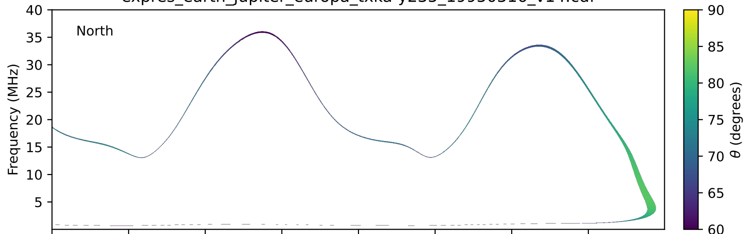
expres_earth_jupiter_europa_txka-y235_19950316_v14.cdf
