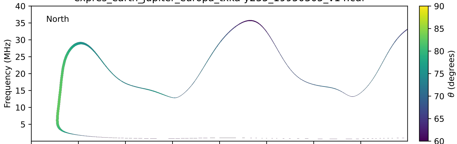
expres_earth_jupiter_europa_txka-y235_19950305_v14.cdf
