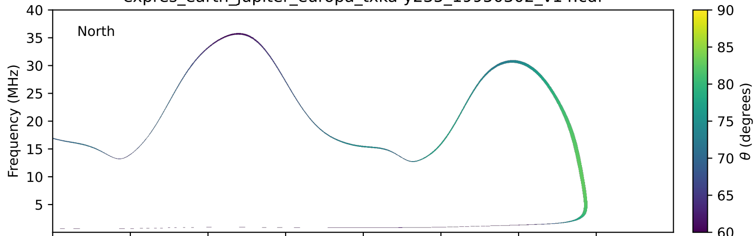
expres_earth_jupiter_europa_txka-y235_19950302_v14.cdf
