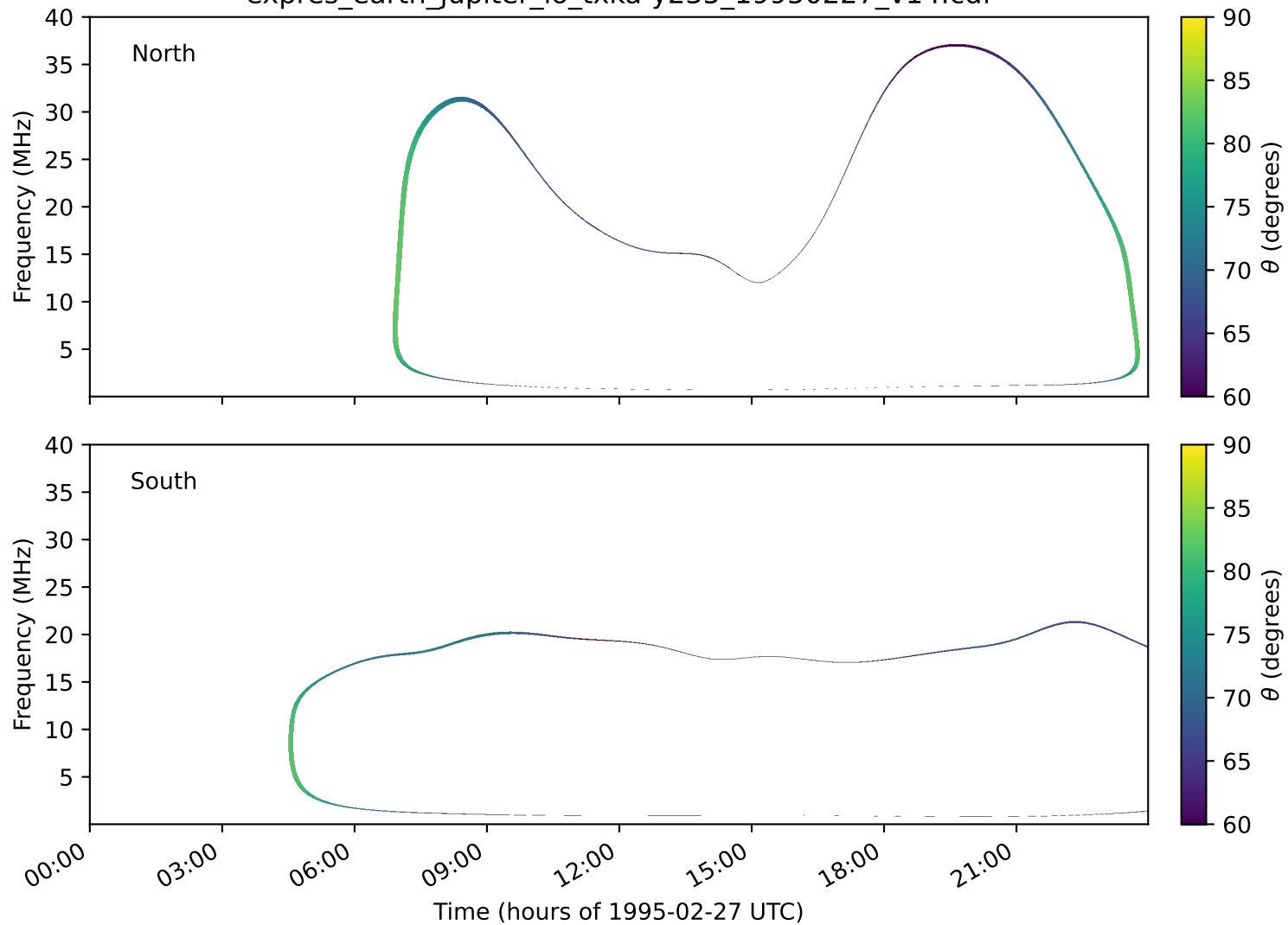
expres_earth_jupiter_io_txka-y235_19950227_v14.cdf
