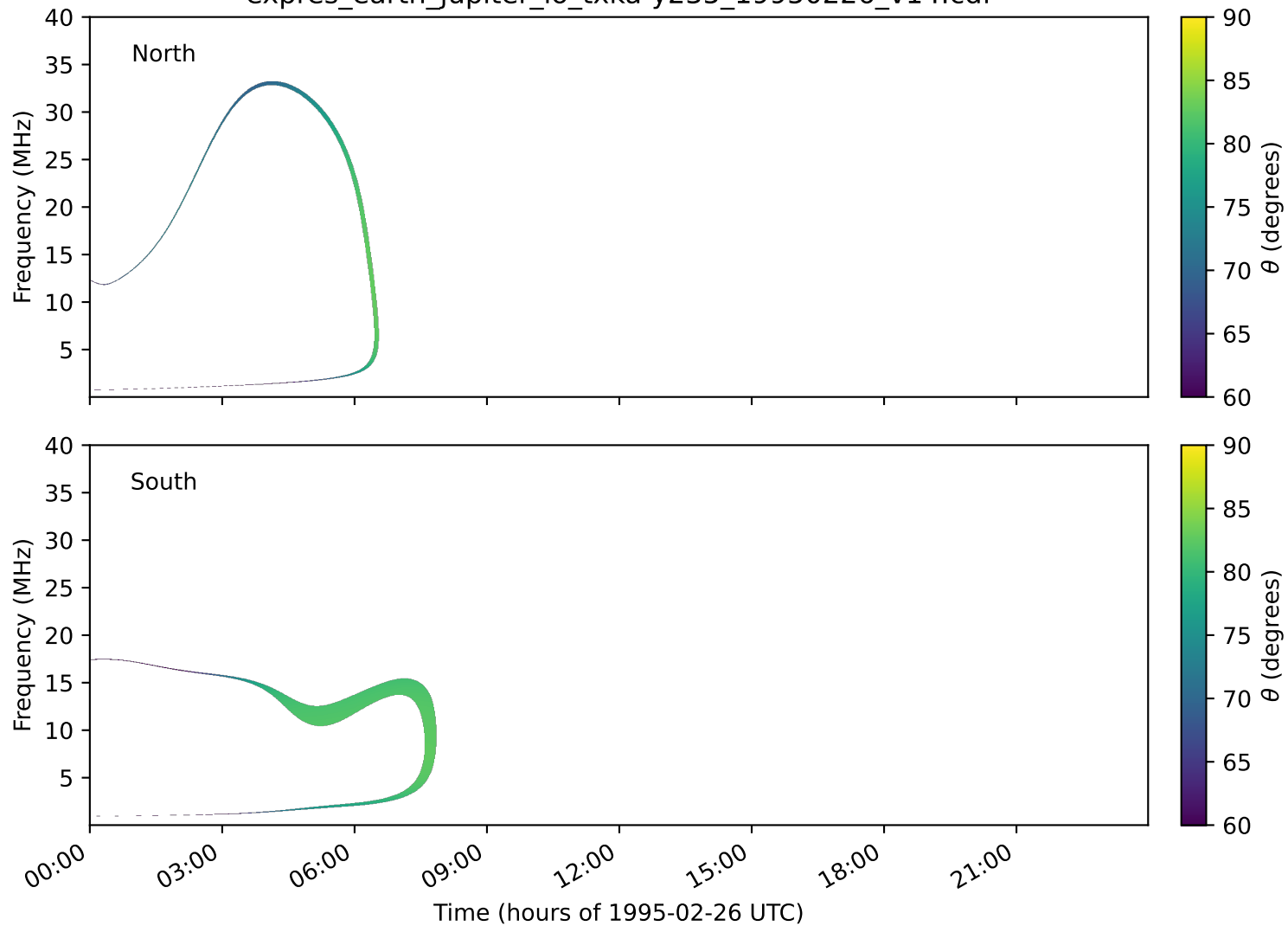
expres_earth_jupiter_io_txka-y235_19950226_v14.cdf
