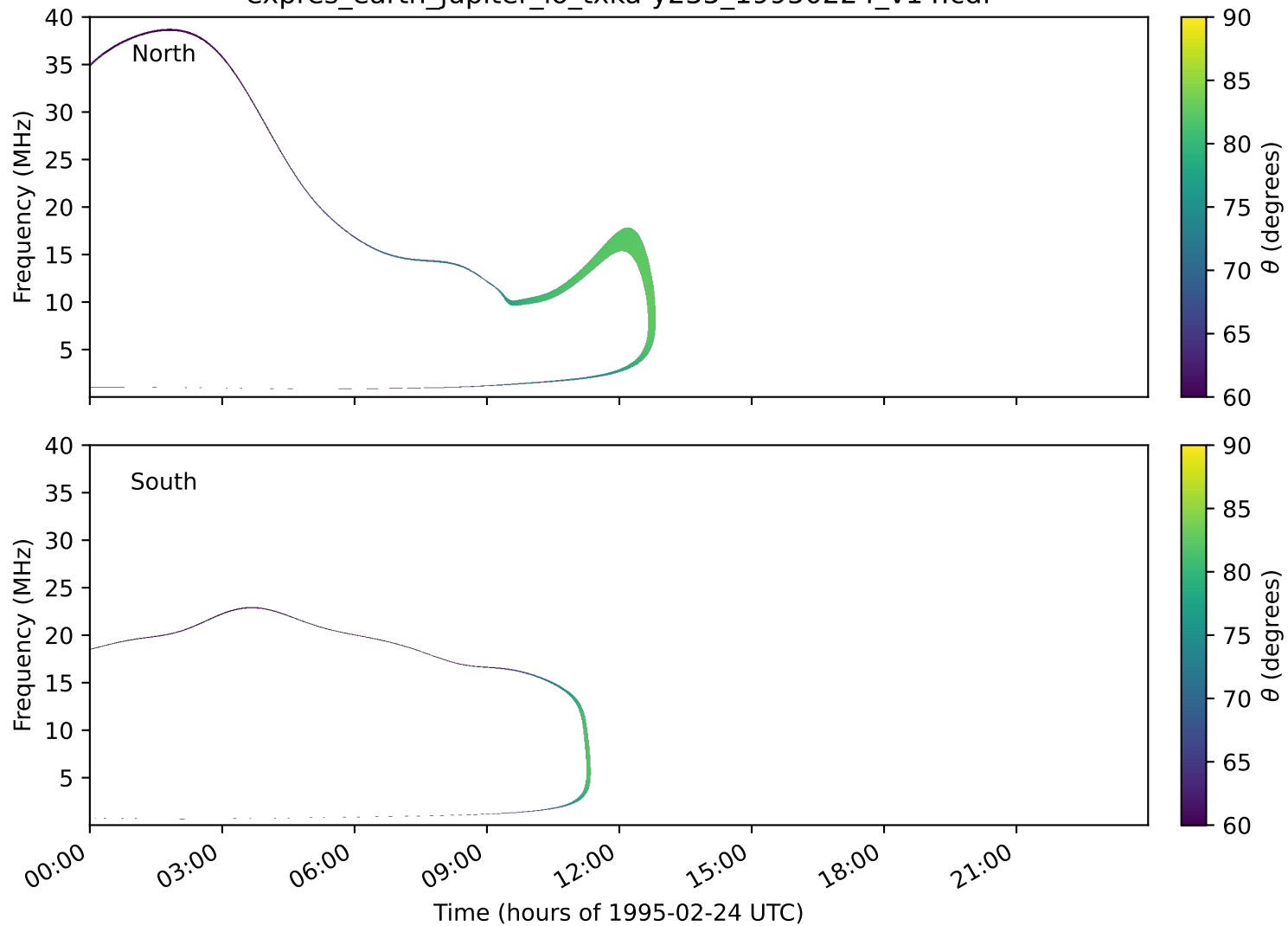
expres_earth_jupiter_io_txka-y235_19950224_v14.cdf
