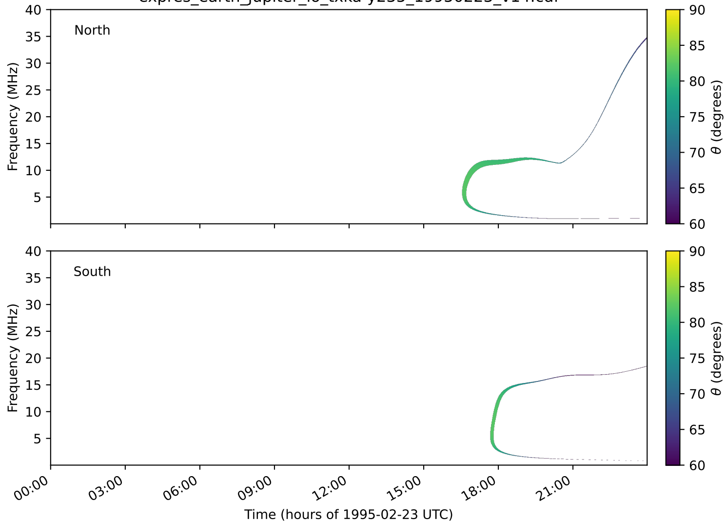
expres_earth_jupiter_io_txka-y235_19950223_v14.cdf
