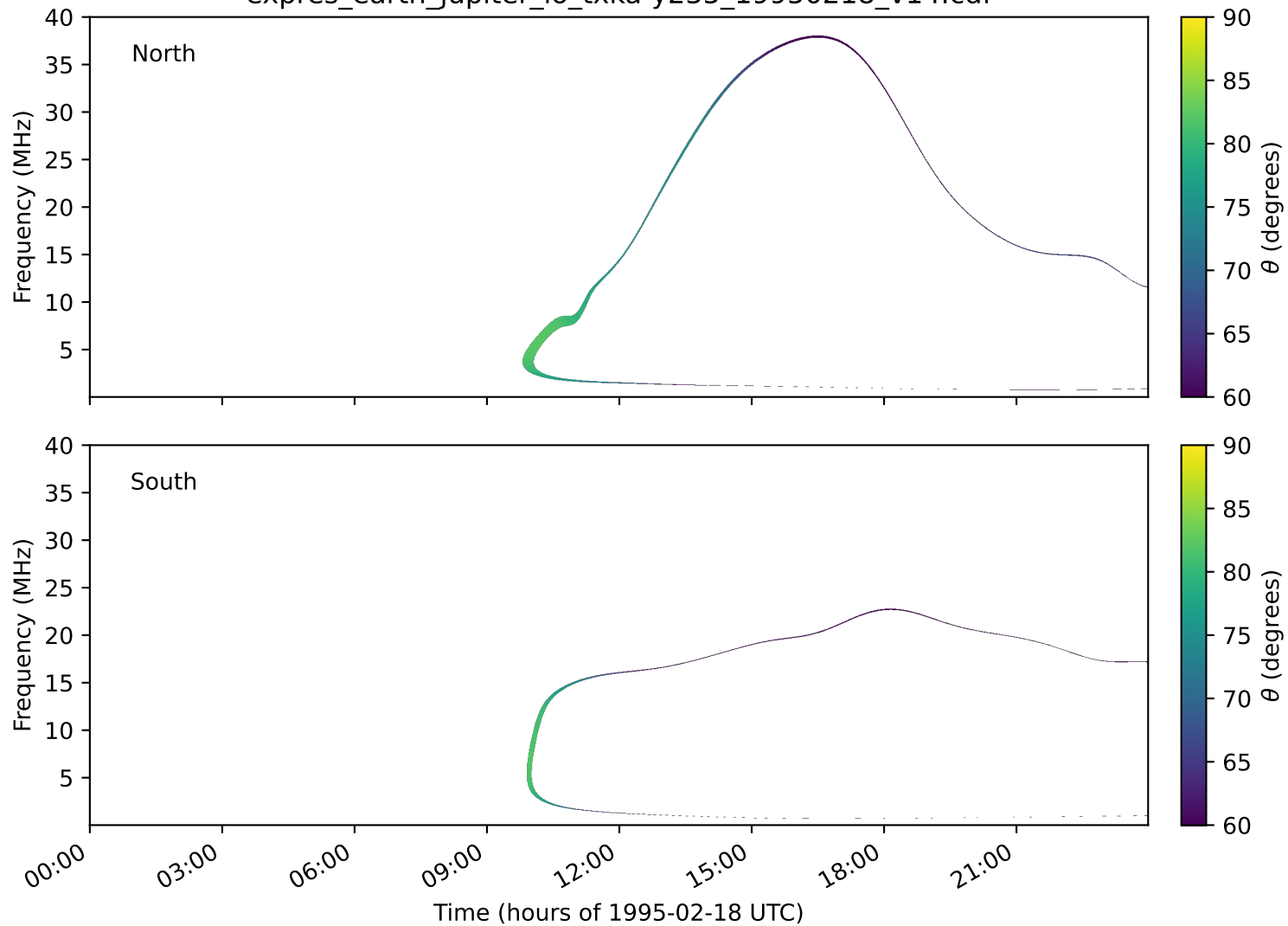
expres_earth_jupiter_io_txka-y235_19950218_v14.cdf
