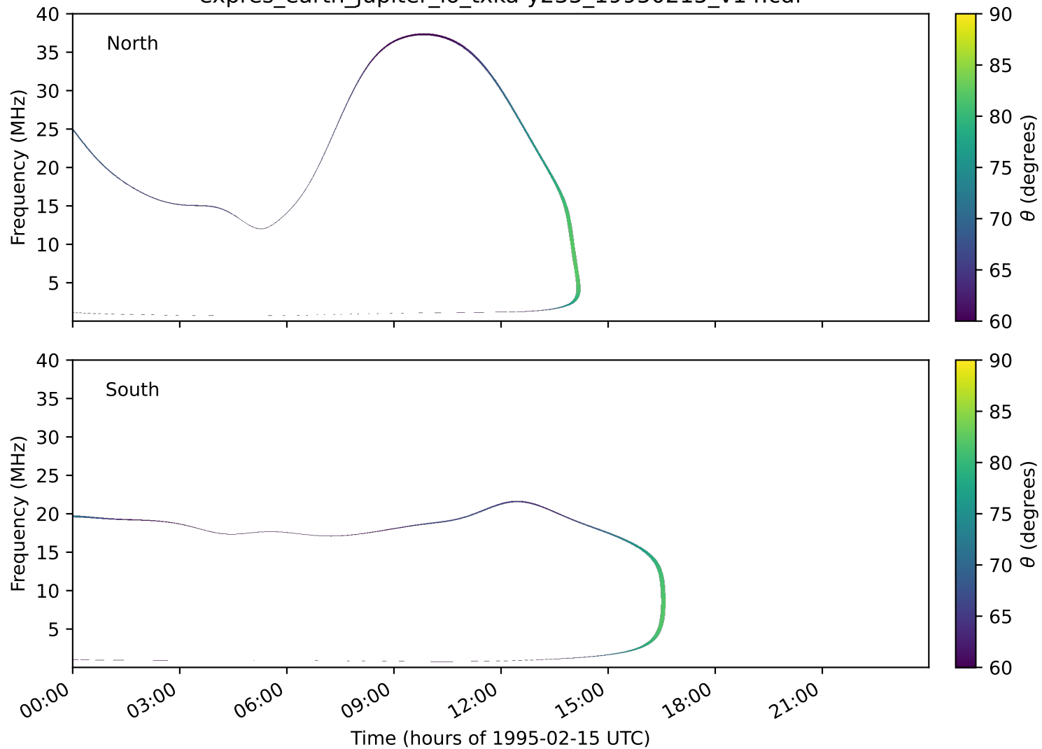
expres_earth_jupiter_io_txka-y235_19950215_v14.cdf
